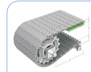
HS-200AN Pitch : 25.4MM Thickness : 11.5MM Open Area : 0%
