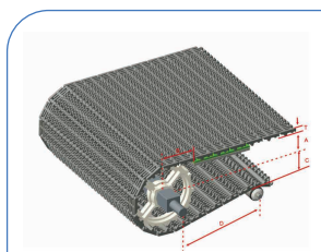
HS-103B-HD-AN Pitch : 50.8MM Thickness : 19MM Open Area : 27%
