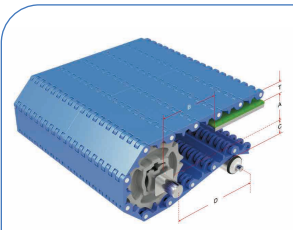
HS-100A-HD Pitch : 50.8MM Thickness : 16MM Open Area : 0%
