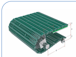
HS-F1000B Pitch : 25.4MM Thickness : 8.6MM Open Area : 42%
