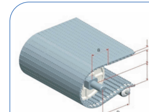
HS-1100A-N Pitch : 15.2MM Thickness : 8.7MM Open Area : 0%
