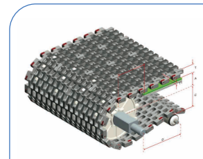
HS-300B-HD-EL Pitch : 45MM Thickness : 18MM Open Area : 38%
