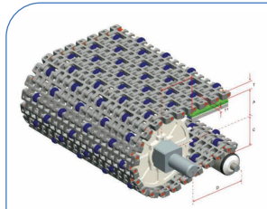
HS-500C Pitch : 25MM Thickness : 13.5MM Open Area : 36%
