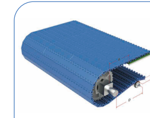
HS-200A-HD Pitch : 25.4MM Thickness : 10.2MM Open Area : 0%
