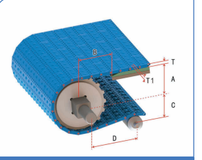
HS-2900C Pitch : 25.4MM Thickness : 12.7MM Open Area : 0%
