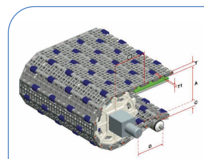
HS-900C Pitch : 50.8MM Thickness : 17MM Open Area : 34%
