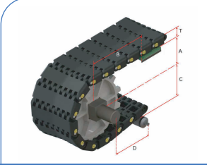
HS-1800E-N Pitch : 63.5MM Thickness : 32MM Open Area : 0%
