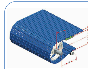
HS-103B-HD Pitch : 50.8MM Thickness : 16MM Open Area : 22%
