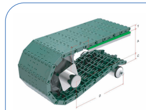
HS-F1000-85AB-GB Pitch : 25.4MM Thickness : 8.6MM Open Area : 1%
