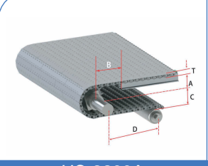
HS-3200A Pitch : 15.2MM Thickness : 8.8MM Open Area : 0%
