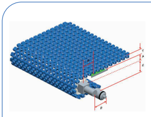
HS-500B-HD Pitch : 25MM Thickness : 12.7MM Open Area : 38%
