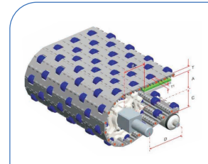
HS-200C Pitch : 25.4MM Thickness : 13MM Open Area : 0%
