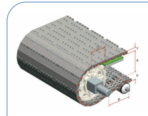
HS-201A Pitch : 25.4MM Thickness : 12.5MM Open Area : 0%
