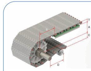
HS-101B-HD Pitch : 50.8MM Thickness : 16MM Open Area : 17.1%
