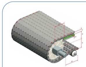
HS-502ZS Pitch : 25MM Thickness : 14.2MM Open Area : 0%
