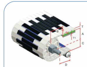
HS-700EL-N Pitch : 27.2MM Thickness : 14.8MM Open Area : 0%
