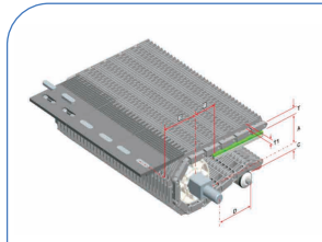
HS-901D Pitch : 50.8MM Thickness : 25.5MM Open Area : 36%
