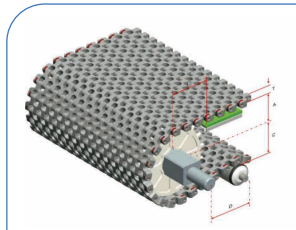
HS-501A Pitch : 25.4MM Thickness : 13MM Open Area : 35%
