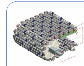
HS-300B-PLUS-C Pitch : 45MM Thickness : 19.5MM Open Area : 52%
