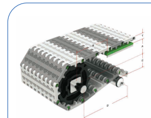
HS-100B-HD-N Pitch : 50.8MM Thickness : 16MM Open Area : 17.6%
