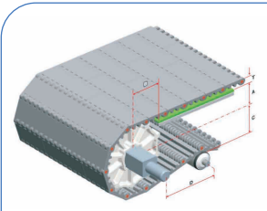
HS-100A Pitch : 50.8MM Thickness : 16MM Open Area : 0%
