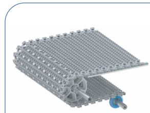
HS-1400B Pitch : 50.8MM Thickness : 14.5MM Open Area : 63%
