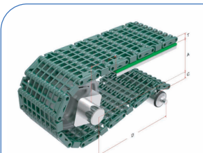
HS-F1000-84B Pitch : 25.4MM Thickness : 8.6MM Open Area : 42%
