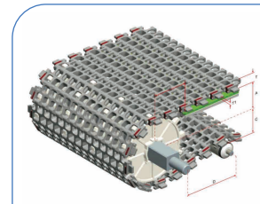
HS-300B-PLUS Pitch : 45MM Thickness : 15MM Open Area : 52%
