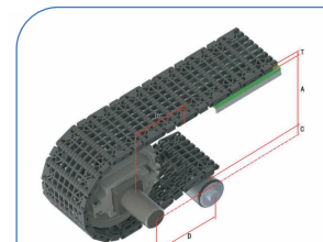
HS-F1000-84B-GB-N Pitch : 25.4MM Thickness : 8.6MM Open Area : 42%
