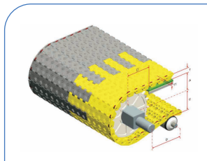
HS-502D Pitch : 25MM Thickness : 14.5MM Open Area : 0%
