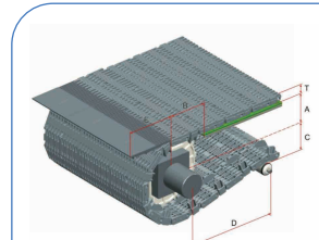
HS-901D-HD Pitch : 50.8MM Thickness : 24MM Open Area : 27%
