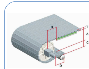
HS-702B-N Pitch : 27.2MM Thickness : 9.8MM Open Area : 24%
