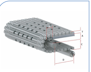
HS-2400B-C Pitch : 25.4MM Thickness : 12.7MM Open Area : 42%
