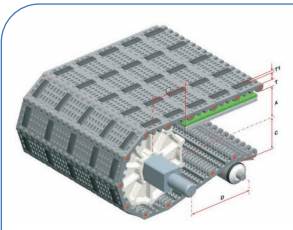
HS-100B-EL Pitch : 50.8MM Thickness : 16MM Open Area : 0%
