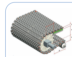
HS-500B Pitch : 25MM Thickness : 11MM Open Area : 36%
