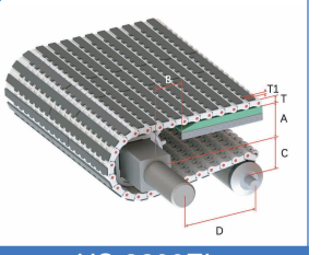
HS-3200EL Pitch : 15.2MM Thickness : 11MM Open Area : 0%
