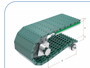
HS-F1000-85A Pitch : 25.4MM Thickness : 8.6MM Open Area : 0%
