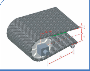
HS-2700D Pitch : 57.15MM Thickness : 24.8MM Open Area : 22.3%
