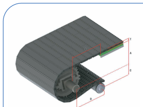
HS-F1000A-N Pitch : 25.4MM Thickness : 8.6MM Open Area : 0%
