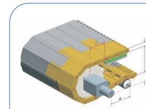
HS-1600A Pitch : 50.8MM Thickness : 20MM Open Area : 0%
