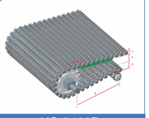
HS-2400B Pitch : 25.4MM Thickness : 12.7MM Open Area : 42%
