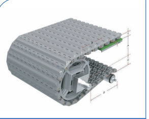
HS-2500E Pitch : 25.4MM Thickness : 13MM Open Area : 0%
