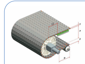
HS-1000A Pitch : 19MM Thickness : 8.5MM Open Area : 0%
