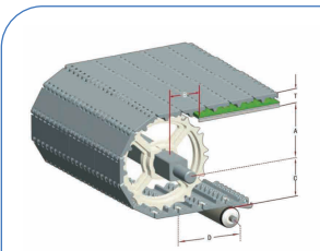
HS-100A-HD-N Pitch : 50.8MM Thickness : 16MM Open Area : 0%
