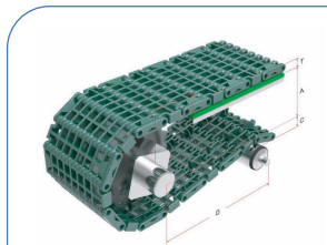
HS-F1000-85B-GB Pitch : 25.4MM Thickness : 8.6MM Open Area : 42%
