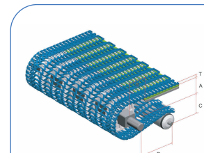
HS-1500B-N Pitch : 12.7MM Thickness : 6.4MM Open Area : 53%
