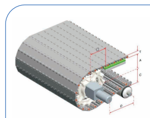
HS-200A Pitch : 25.4MM Thickness : 10MM Open Area : 0%
