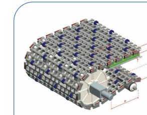
HS-300C Pitch : 45MM Thickness : 19.5MM Open Area : 52%
