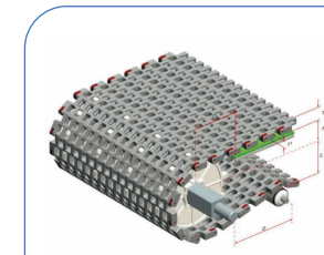
HS-300B-HD-GB Pitch : 45MM Thickness : 15MM Open Area : 38%
