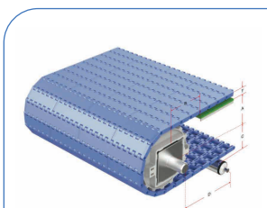
HS-502A-HD Pitch : 25.4MM Thickness : 8.8MM Open Area : 0%
