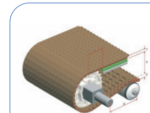
HS-1500A-HD Pitch : 12.7MM Thickness : 10MM Open Area : 0%
