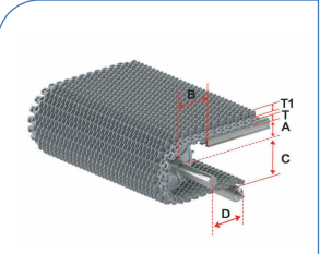
HS-2400D Pitch : 25.4MM Thickness : 25.4MM Open Area : 42%
