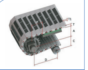
HS-2500EL Pitch : 25.4MM Thickness : 14MM Open Area : 0%
