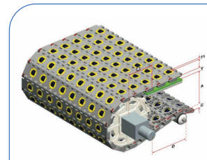
HS-800-1C Pitch : 50.8MM Thickness : 18MM Open Area : 0%
