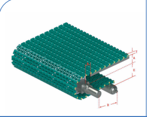
HS-2500B Pitch : 25.4MM Thickness : 10MM Open Area : 31.7%
