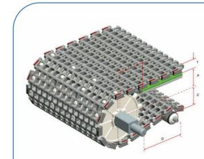
HS-300B Pitch : 45MM Thickness : 15MM Open Area : 52%
