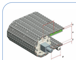
HS-900B Pitch : 50.8MM Thickness : 14MM Open Area : 34%
