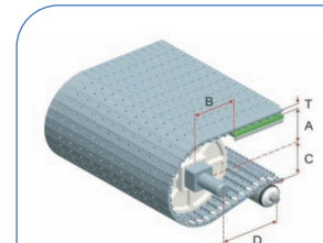
HS-1100AB-N Pitch : 15.2MM Thickness : 8.7MM Open Area : 3%
