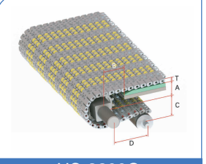
HS-3200C Pitch : 15.2MM Thickness : 11.5MM Open Area : 13%
