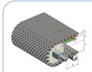
HS-600B Pitch : 25.4MM Thickness : 18MM Open Area : 0%
