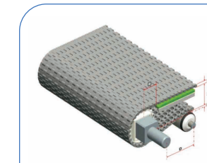
HS-400A Pitch : 10MM Thickness : 7MM Open Area : 0%
