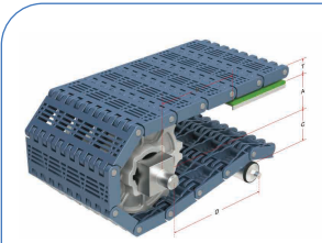
HS-902B Pitch : 50.8MM Thickness : 16MM Open Area : 23%
