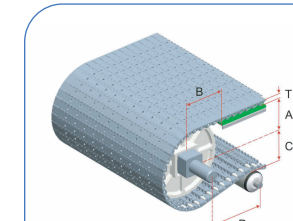
HS-1100B-N Pitch : 15.2MM Thickness : 8.7MM Open Area : 28%
