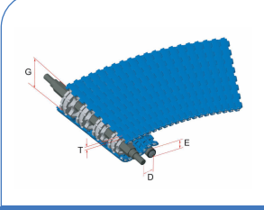
HS-2000A-RC Pitch : -- Thickness : 10MM Open Area : 0%
