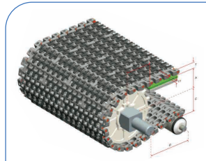
HS-500EL Pitch : 25MM Thickness : 15.5MM Open Area : 36%
