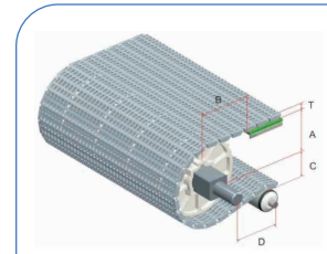
HS-700B-N Pitch : 27.2MM Thickness : 8.7MM Open Area : 38%
