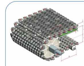
HS-300B-PLUS-EL Pitch : 45MM Thickness : 18MM Open Area : 52%
