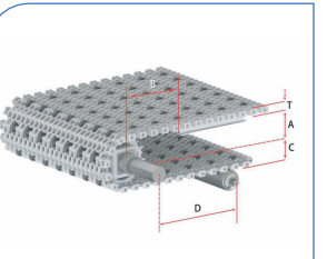
HS-2400B-2.2-C Pitch : 25.4MM Thickness : 12.7MM Open Area : 42%
