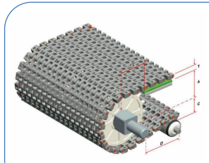
HS-500B-GB Pitch : 25MM Thickness : 11MM Open Area : 36%
